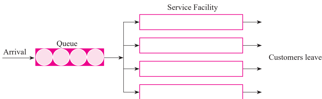
Figure 4.2 (b): Multiple, Parallel Servers, Single Queue Model
