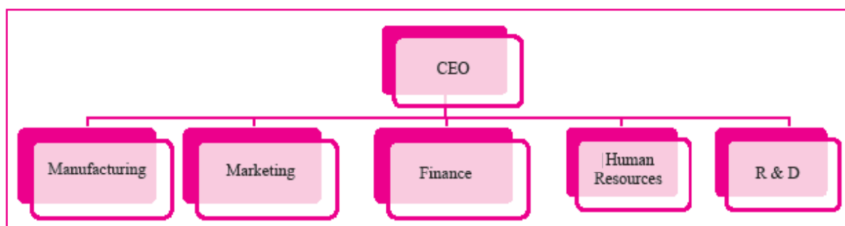
Figure 10.1: Functional Structure
