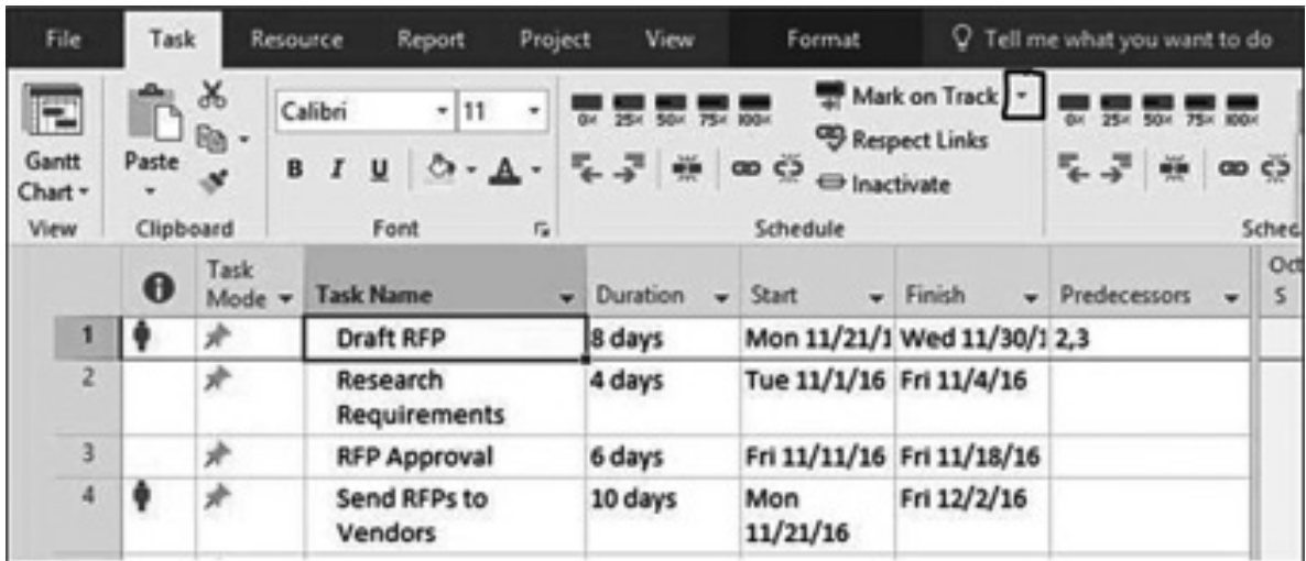
Figure 6.18: MS Project - 18
