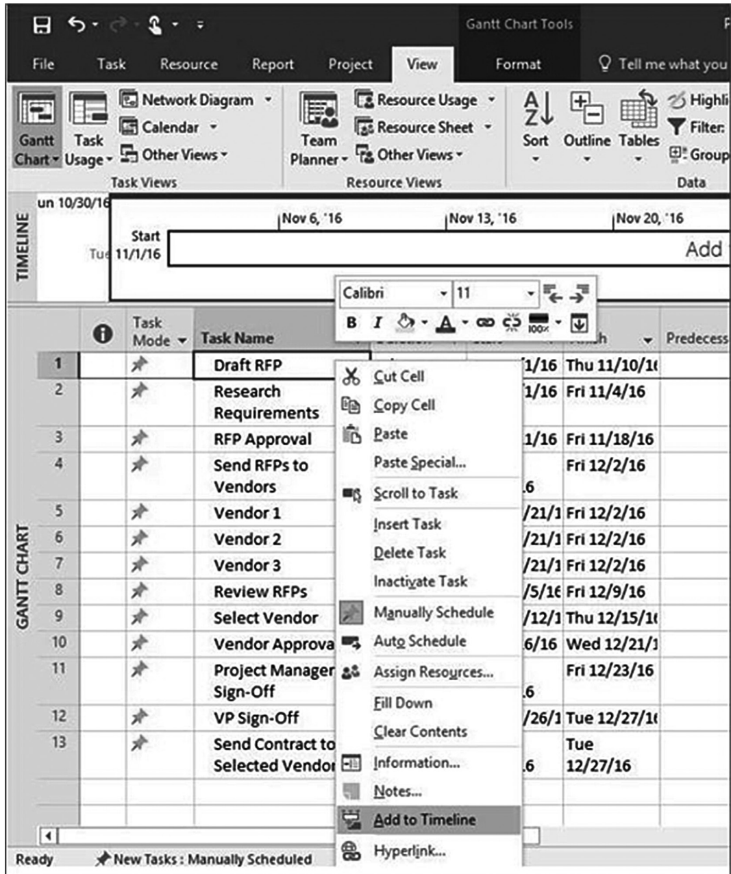
Figure 6.4: MS Project - 4
