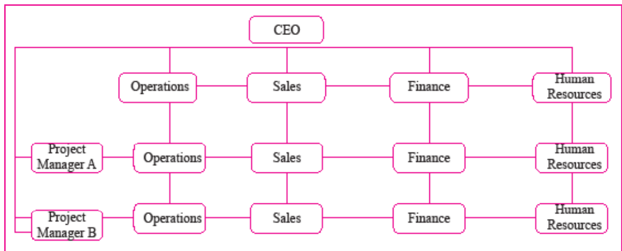
Figure 10.3: Matrix Structure
